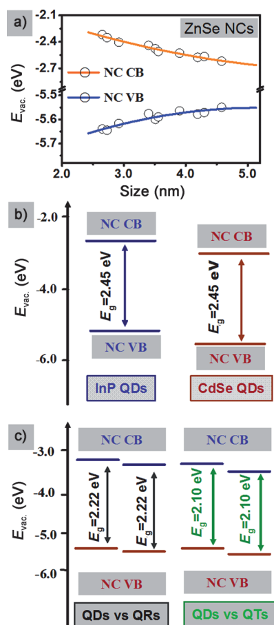
Figure 3. a) Variations in the energy levels of the ZnSe NCs with size. b) Energy levels of the InP (2.0 nm) and CdSe (2.4 nm) dots with the same energy gap (505 nm, E_g = 2.45 eV). c) Energy levels of the CdSe dots (3.2 nm) versus CdSe rods (diameter \times length: 3.2 \times 7.5 nm) with the same energy gap (558 nm, E_g = 2.22 eV) (left), and CdSe dots (4.0 nm) versus CdSe tetrapods (diameter \times arm length: 4.0 \times 28 nm) with the same energy gap (583 nm, E_g = 2.10 eV) (right).
